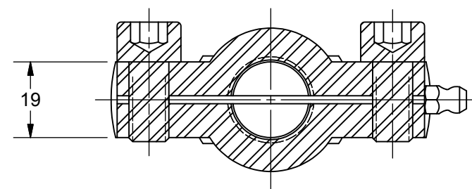
SECTION A-A SCALE .75
