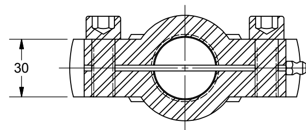
SECTION A-A SCALE .5
