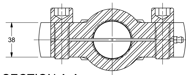
SECTION A-A SCALE .5
