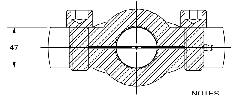
SECTION A-A SCALE .38
